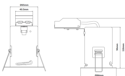
IP65 Showerlight Cut-Out: 69mm
